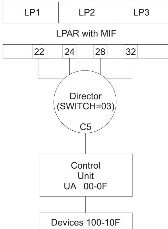
Figure 35. LPAR mode with shared paths to an ESCON device
