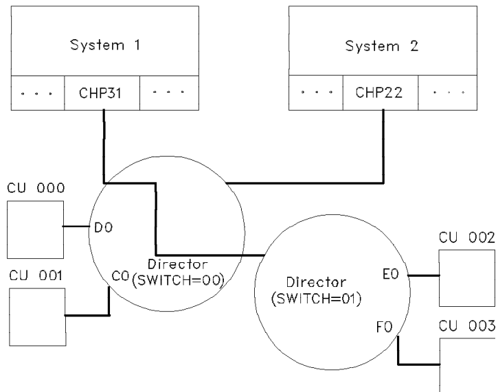
Figure 39. Chained ESCON directors
