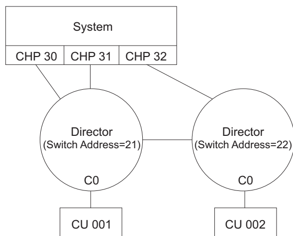
Figure 40. Cascaded FICON directors
