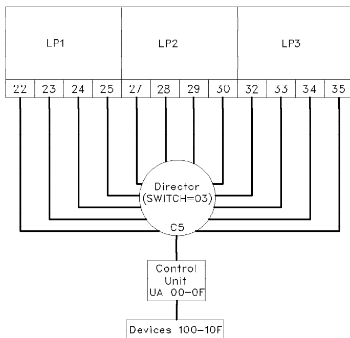
Figure 34. LPAR mode with more than eight paths to an ESCON device
