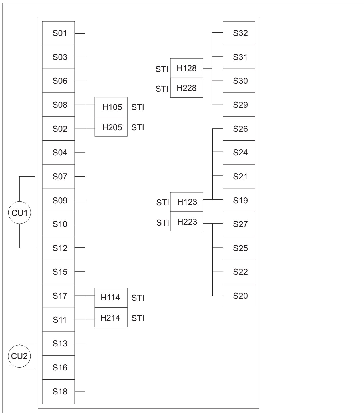
Figure 6. I/O channel path configuration for a representative I/O cage in a 2094 or 2096 model
