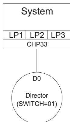
Figure 38. FICON CTC and director with single path
