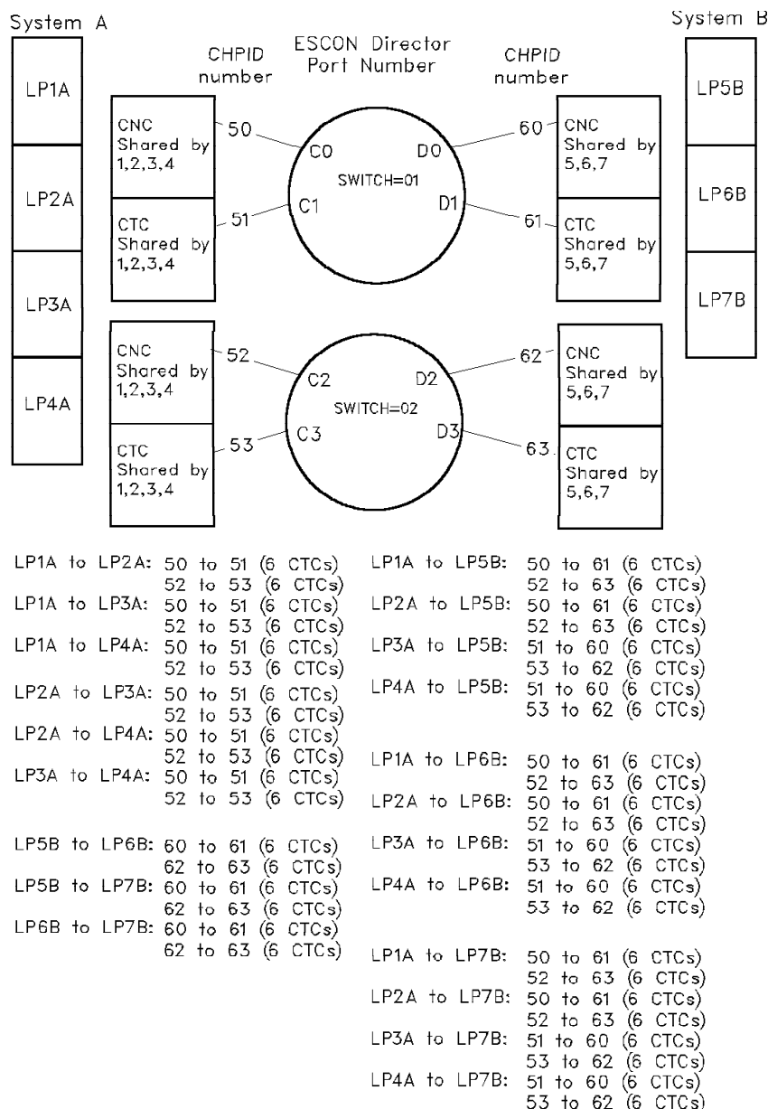
Figure 50. ESCON CTC with shared channels
