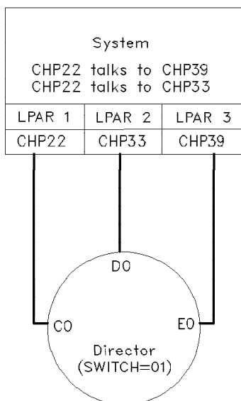
Figure 37. ESCON CTC dynamic through an ESCON director with multiple paths
