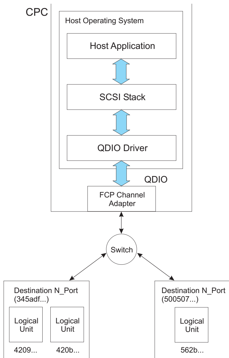
Figure 47. FCP channel configuration
