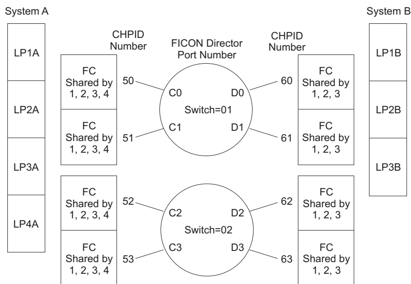
Figure 51. FICON CTC (fully redundant)
