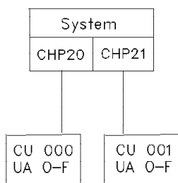
Figure 44. ESCON control units requiring unit address 00
