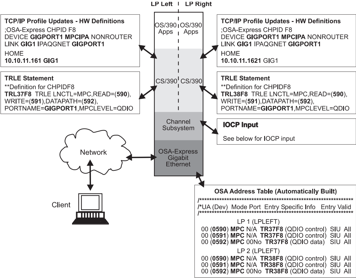
Figure 45. OSA configuration with two logical partitions
