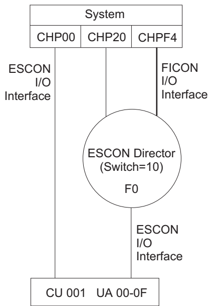
Figure 43. FCV channel configuration
