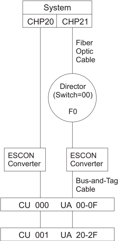
Figure 42. Channels through an ESCON converter
