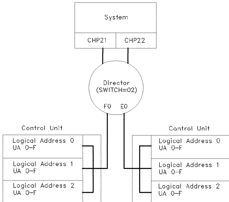
Figure 41. Control unit logical addressing
